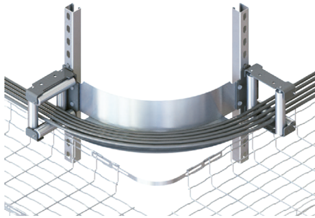
6" Radius cable guide is useful in tight radius bends for copper cabling.
