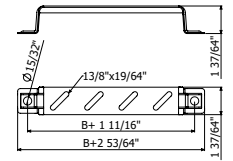
SV 4" / 6" / 8" / 12"
